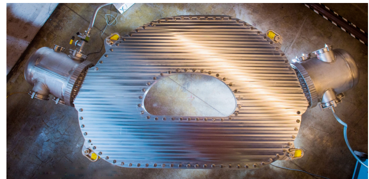
Commonwealth Fusion Systems and MIT announced achievement of 20T large bore HTSC coil
